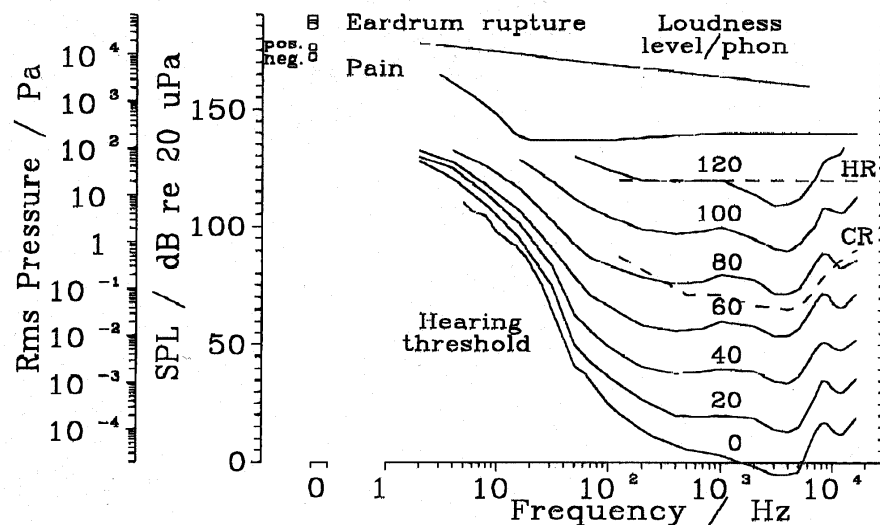
Fig. 2 Threshold of hearing (corresponding to 0 phone), curves of equal perceived loudness for 20, 40, 60, 80, 100, and 120 phones, rms sound pressure (logarithmic scale) and its level versus frequency. The threshold values are for binaural hearing of pure tones; monaural perception thresholds are higher. Also given are the thresholds of conditional (CR) and high (HR) risk of permanent hearing loss (dashed), of aural pain and of eardrum rupture. The high-risk threshold is also valid for the feeling of discomfort; the threshold for tickle sensation is slightly below the one for pain. Especially for eardrum rupture, the threshold is only roughly known. On the left, pain and eardrum rupture thresholds are shown for static pressure. For pain, the values for over-(pos.) and underpressure (neg.) are slightly different. Note that normal atmospheric pressure is 101 kPa. 63
